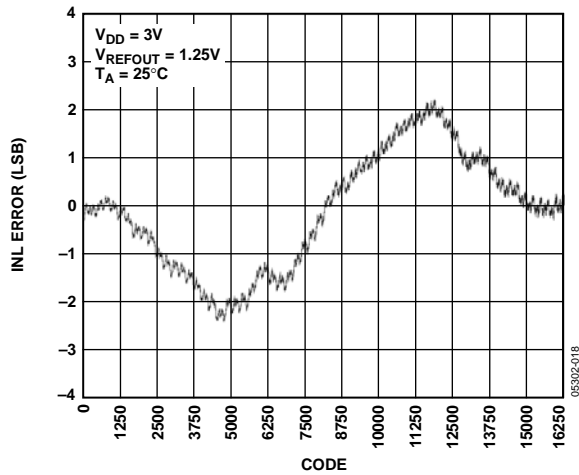
Figure 18. INL AD5648-1
